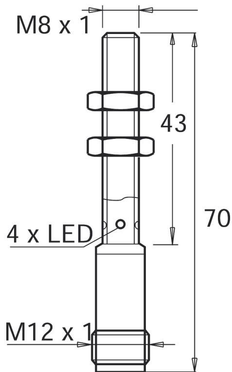
Dimension Diagram
